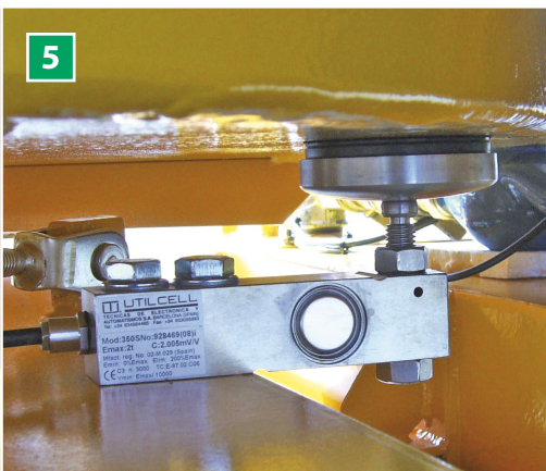
5 Load cells The pan mixer is placed on three electronic load cells with an accuracy of less than +/- 0.5%.
