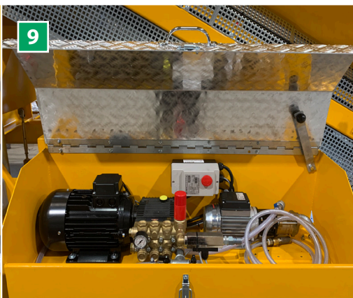
9 Equipment Standard bogie models are delivered with a high-pressure cleaner, while additive pumps are optional.
