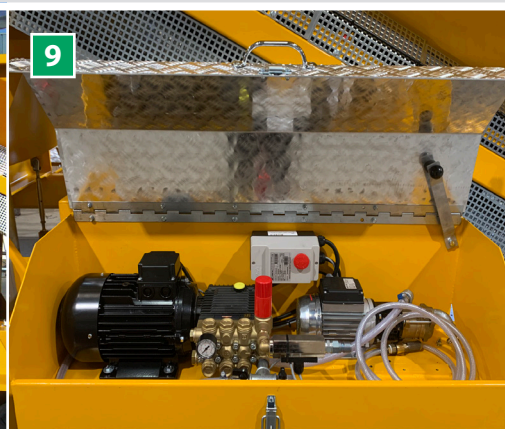
9 Equipment The standard F-model is delivered with a high pressure cleaner while the additive pumps are optional.
