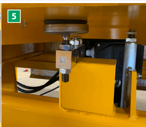
5 Load cells The pan mixer is placed on three 5000 kg electronic load cells with an accuracy of +/- 0,5 %.
